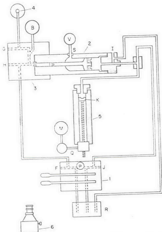
Fig. 1 - Schematic drawing of the high-pressure apparatus.
